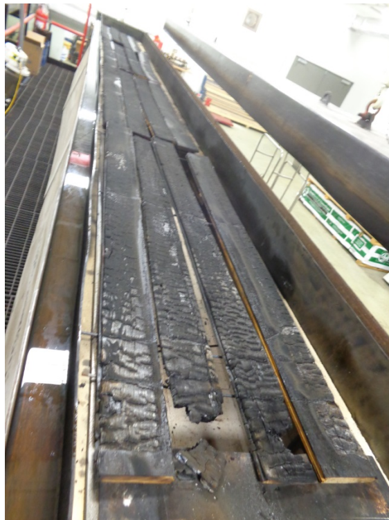
Photo No. 2 Exposed Surface (Post-test)
